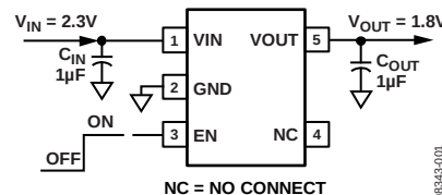
Figure 1. 5-Lead TSOT with Fixed Output Voltage, 1.8 V
