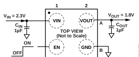
Figure 2. 4-Ball WLCSP with Fixed Output Voltage, 1.8 V
