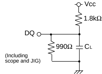
Fig.1 Output load
