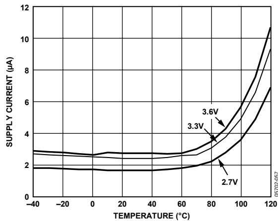
Figure 15. Shutdown Supply Current vs. Temperature (Supply Current = I_{CC} + D I_{CC} )
