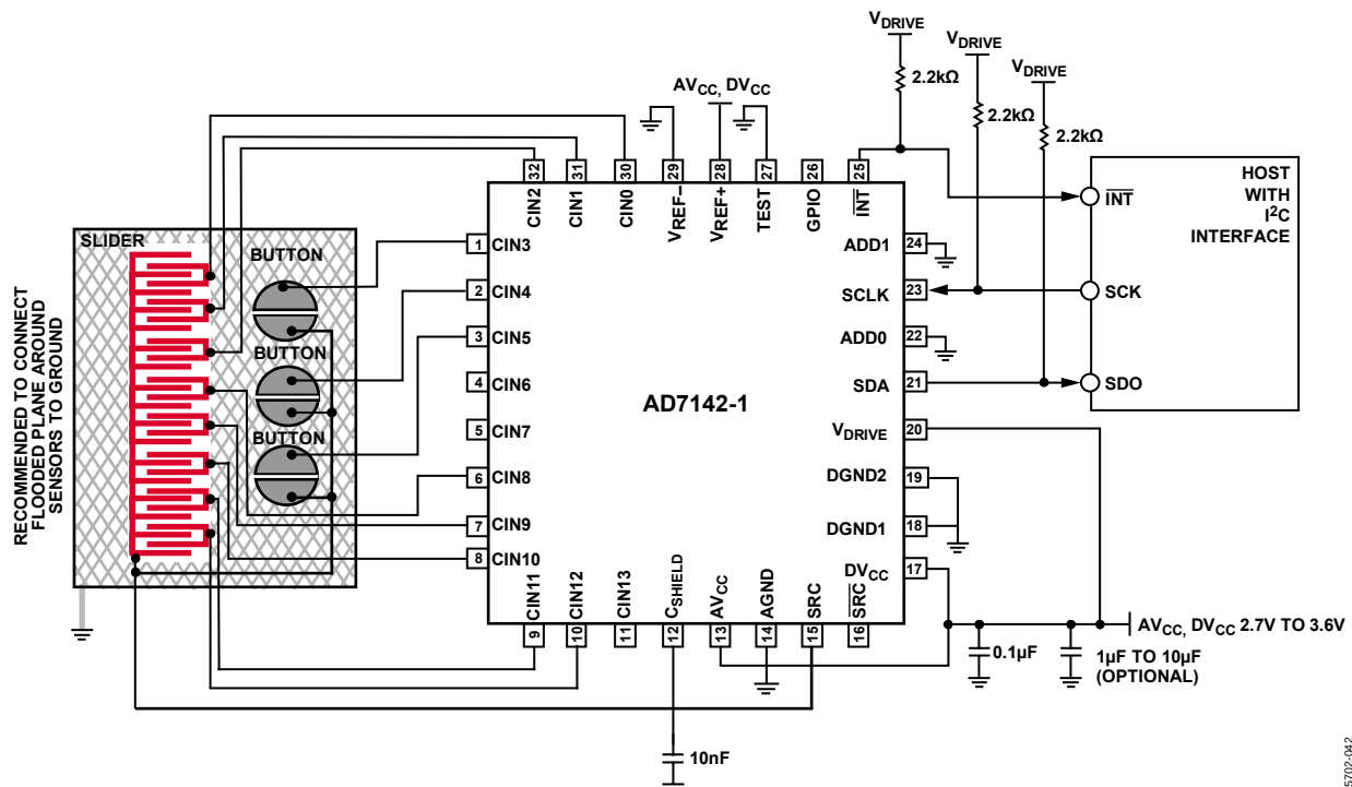
Figure 58. Typical Application Circuit with I²C Interface
