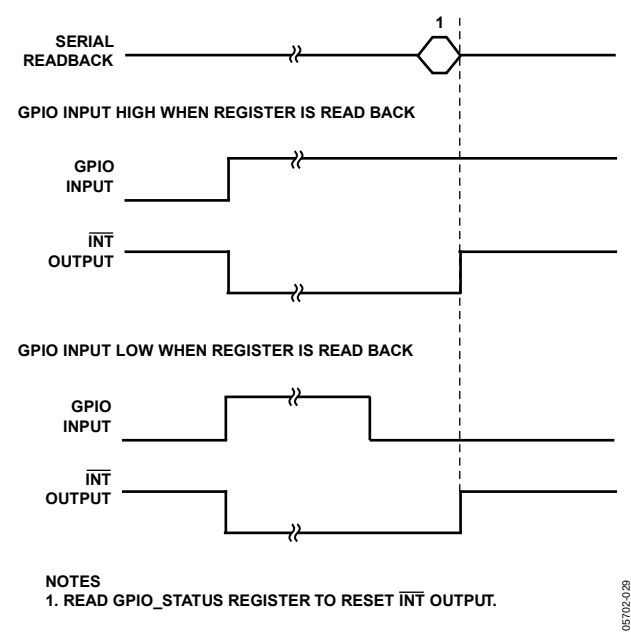
Figure 42. INT Output Controlled by the GPIO Input Example, GPIO_SETUP = 01, GPIO_INPUT_CONFIG = 01
