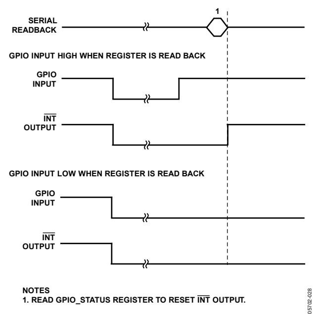
Figure 41. INT Output Controlled by the GPIO Input Example, GPIO_SETUP = 01, GPIO_INPUT_CONFIG = 00
