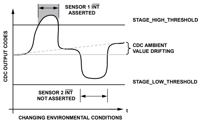
Figure 34. Typical Sensor Behavior Without Calibration Applied
