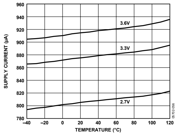
Figure 14. Supply Current vs. Temperature (Supply Current = I_{CC} + D I_{CC} )
