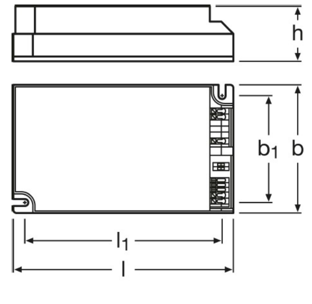
Product line drawing OT 35/220...240/700 LTCS
