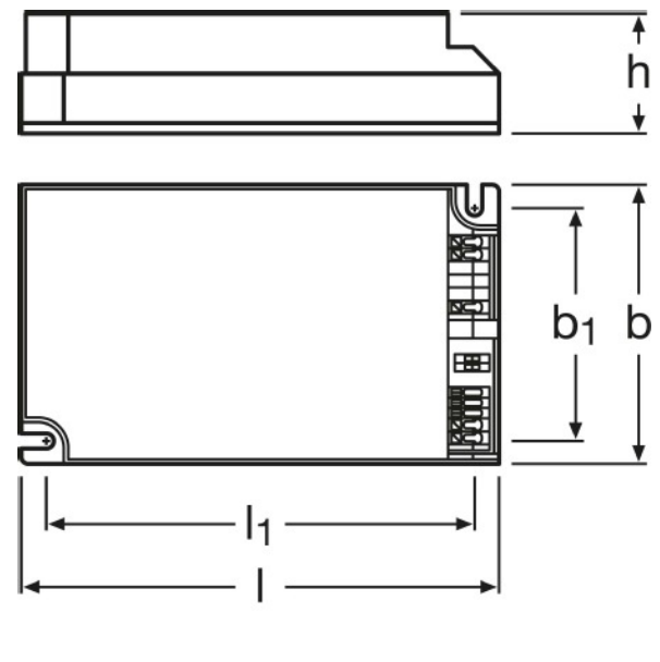
Product line drawing OT 45/220...240/700 LTCS
