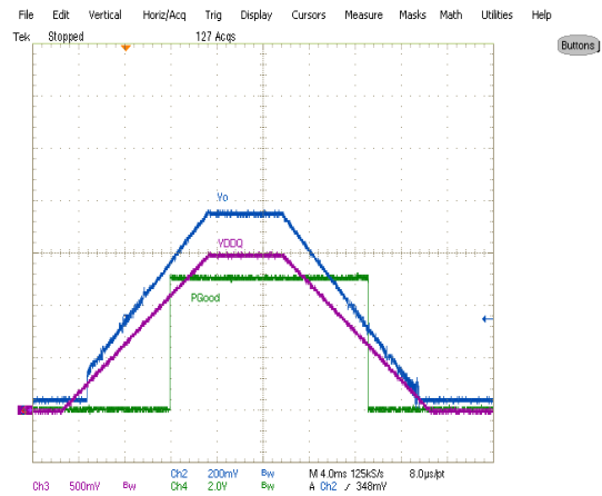
Fig. 23: Tracking -3A load, sinking current, Ch_2: V_{out} , Ch_3: I_L , Ch_4: V_{DDQ} , Ch_5: PGood
