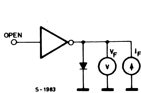
Figure 10. Clamp diode forward voltage
