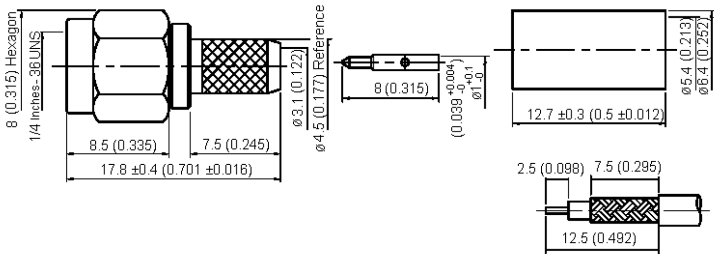
Stripping Dimension
