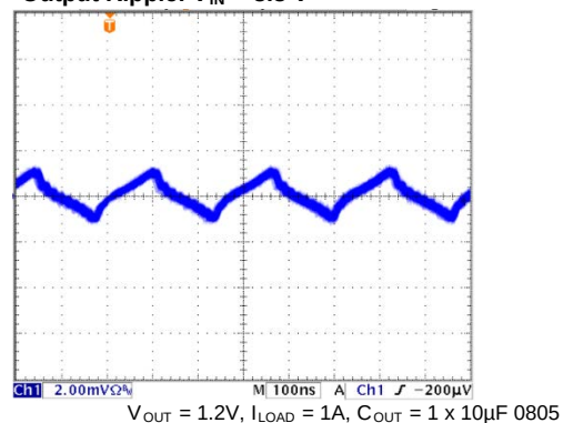
Output Ripple: V_{IN} = 3.3V
