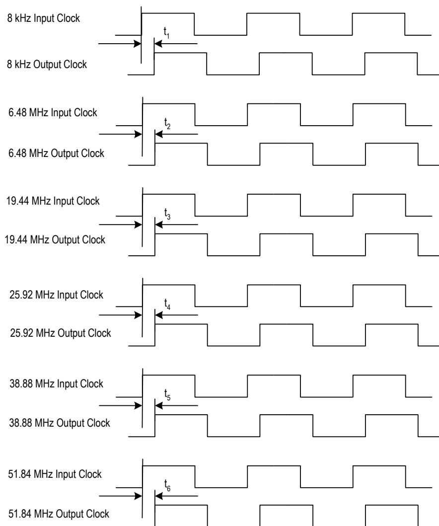
Figure 33. Input / Output Clock Timing
