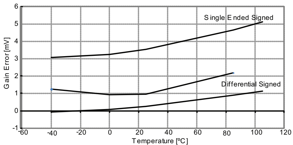
Figure 37-127. Gain error vs. temperature.
