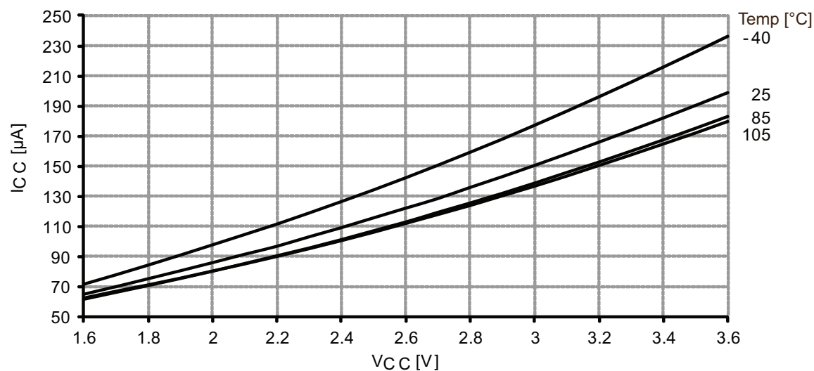
Figure 37-3. Active mode supply current vs. V_{CC} . f_{SYS} = 32.768\text{kHz} internal oscillator.
