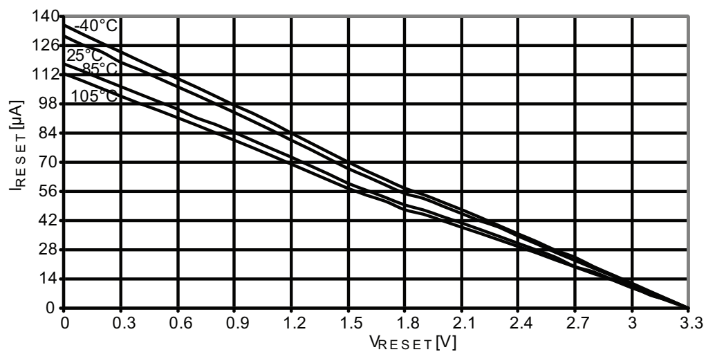
Figure 37-313. Reset pin pull-up resistor current vs. reset pin voltage.
