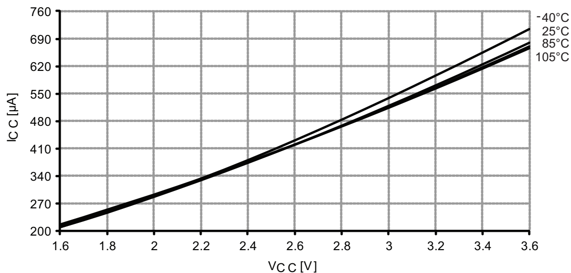
Figure 37-4. Active mode supply current vs. V_{CC} . f_{SYS} = 1\text{MHz} external clock.
