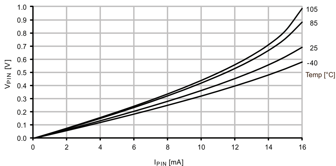
Figure 37-111. I/O pin output voltage vs. sink current.
