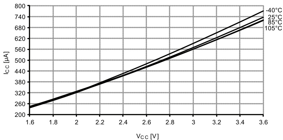
Figure 37-170. Active mode supply current vs. V_{CC} .
