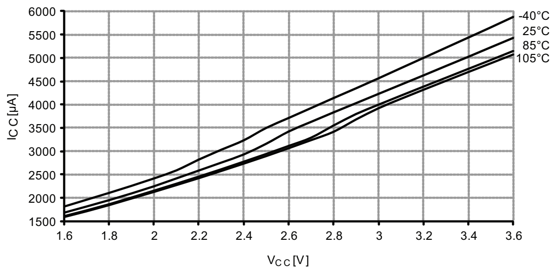
Figure 37-255. Active mode supply current vs. V_{CC} .
