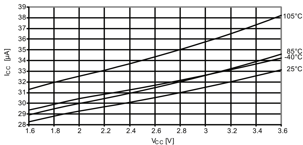
Figure 37-176. Idle mode supply current vs. V_{CC} .
