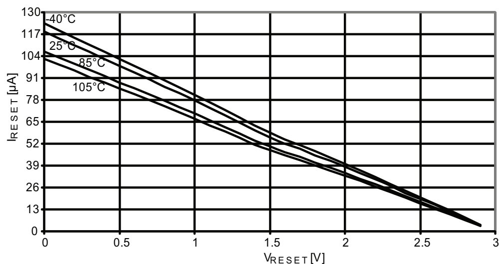
Figure 37-312. Reset pin pull-up resistor current vs. reset pin voltage.
