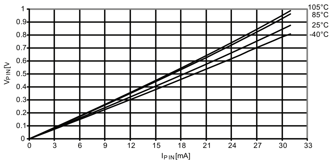
Figure 37-196. I/O pin output voltage vs. sink current.
