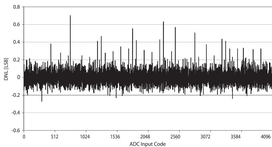
Figure 37-206. DNL error vs. input code.
