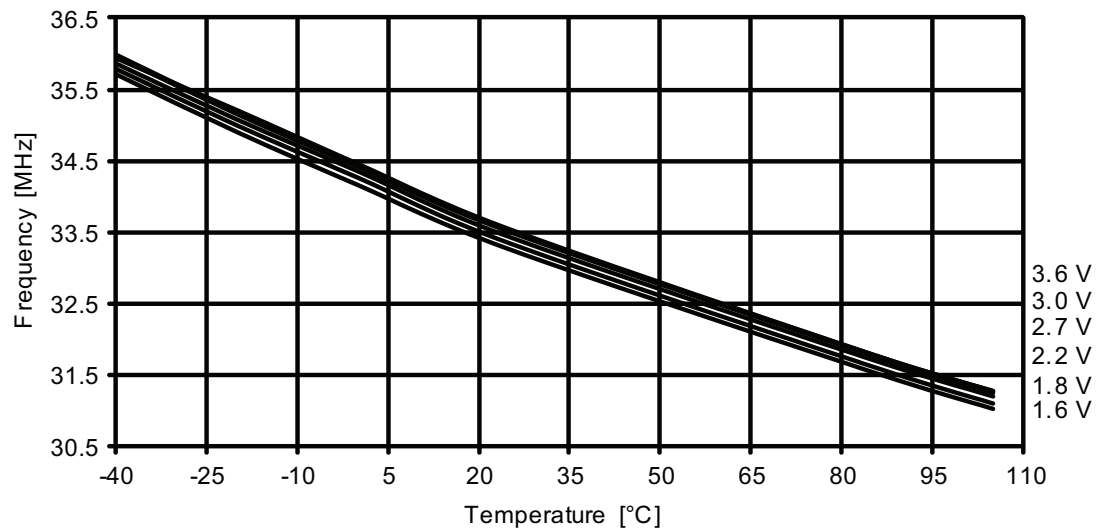
Figure 37-240. 32MHz internal oscillator frequency vs. temperature. DFLL disabled.
