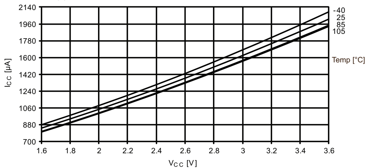
Figure 37-97. Idle mode current vs. V_{CC} .
