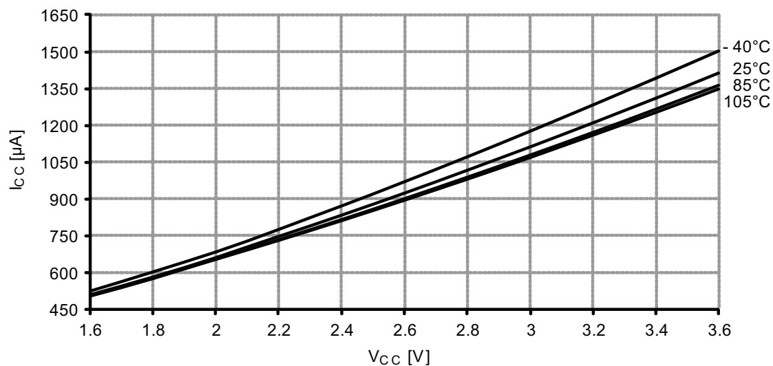
Figure 37-254. Active mode supply current vs. V_{CC} .
