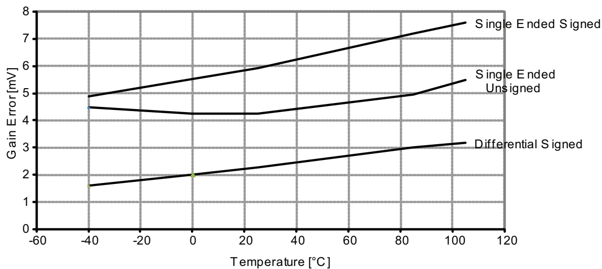
Figure 37-44. Gain error vs. temperature.
