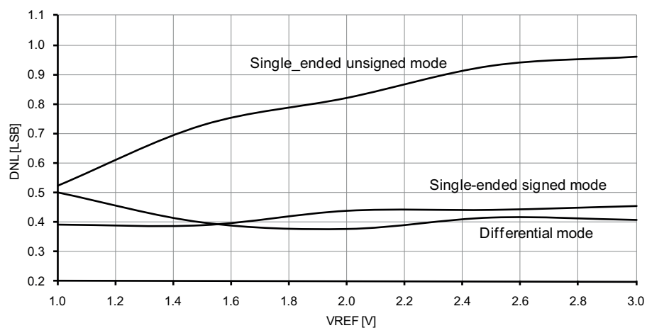
Figure 37-38. DNL error vs. external V_{REF} . T = 25^{\circ}\text{C} , V_{CC} = 3.6\text{V} , external reference.
