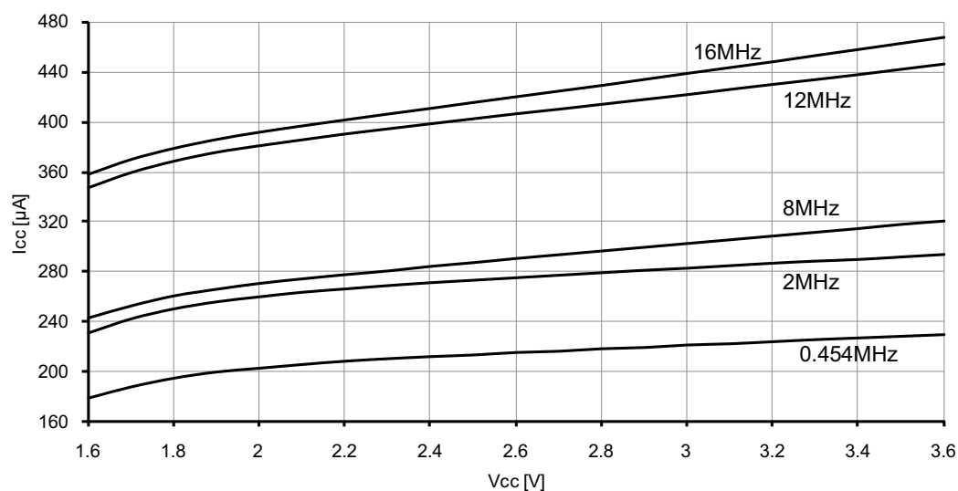
Figure 37-19. Standby supply current vs. V_{CC} . 25°C, running from different crystal oscillators.
