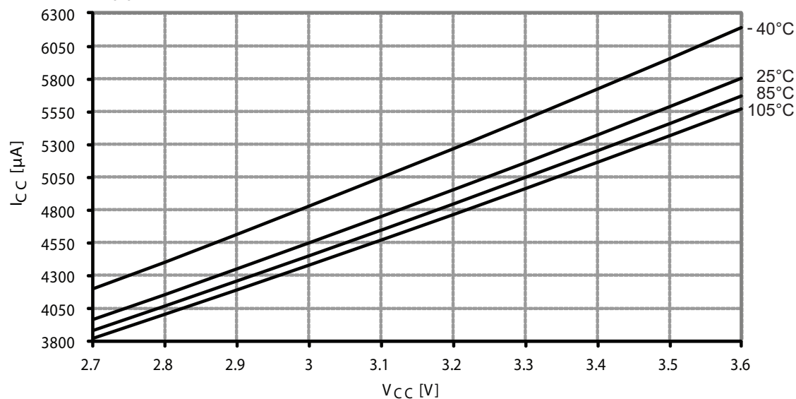
Figure 37-14. Idle mode current vs. V_{CC} . f_{SYS} = 32\text{MHz} internal oscillator.
