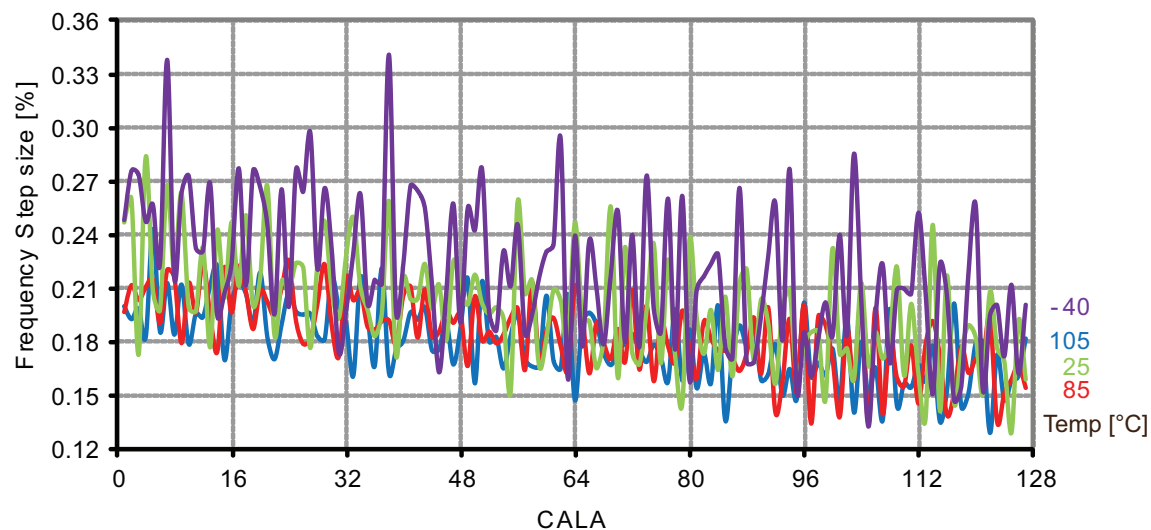
Figure 37-80. 48MHz internal oscillator CALA calibration step size.
