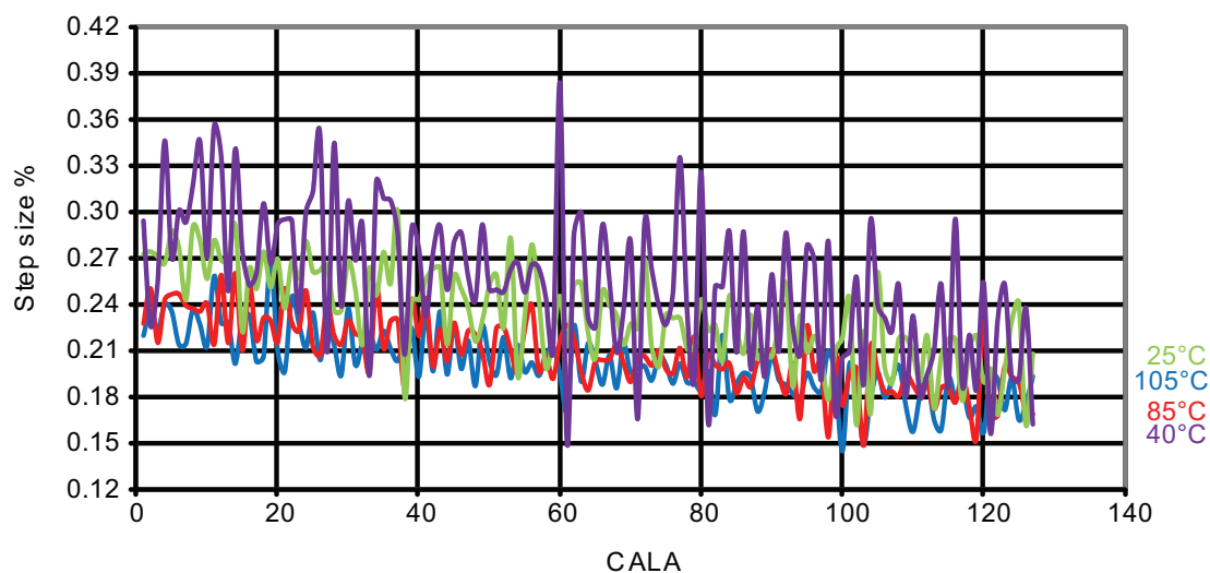
Figure 37-246. 48MHz internal oscillator CALA calibration step size.
