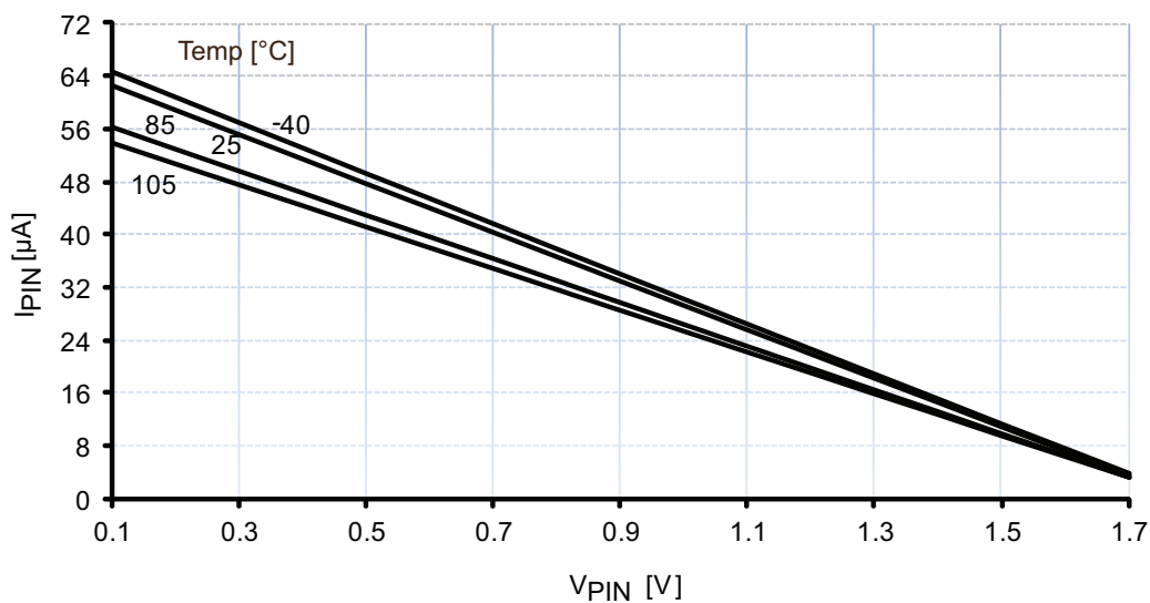
Figure 37-20. I/O pin pull-up resistor current vs. input voltage. V_{CC} = 1.8V .
