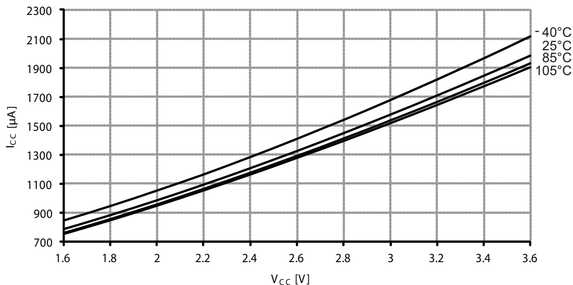
Figure 37-13. Idle mode supply current vs. V_{CC} . f_{SYS} = 32\text{MHz} internal oscillator prescaled to 8MHz.
