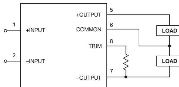
Figure 3c. Fixed-Value Trim Up Resistor
