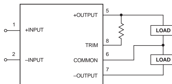
Figure 3b. Fixed-Value Trim Down Resistor
