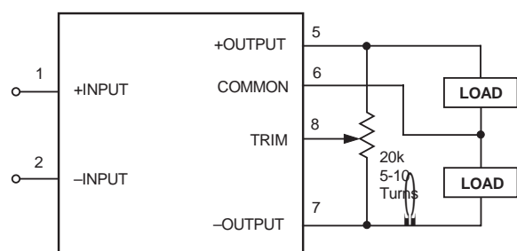
Figure 3a. Trim Connections Using a Trimpot
