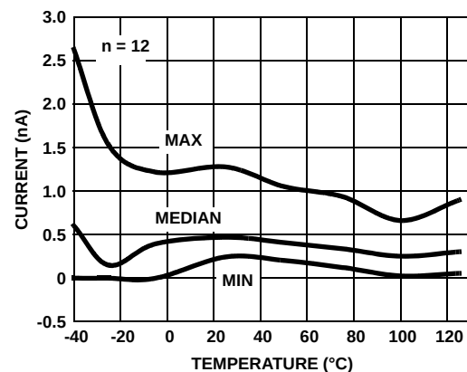
FIGURE 31. I_{\text{BIAS}} (-) vs TEMPERATURE V_S = \pm 1.2V
