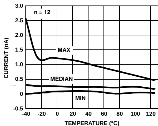
FIGURE 29. I_{\text{BIAS}} (+) vs TEMPERATURE V_S = \pm 1.2V
