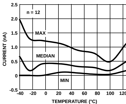
FIGURE 30. I_{\text{BIAS}} (-) vs TEMPERATURE V_S = \pm 2.5V
