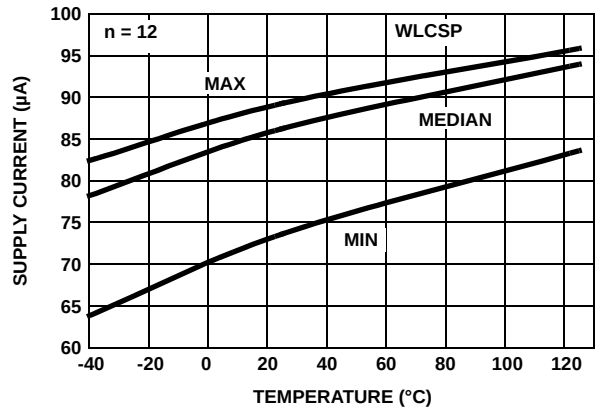
FIGURE 26. SUPPLY CURRENT vs TEMPERATURE V_S = \pm 2.5V ENABLED. R_L = \text{INF}
