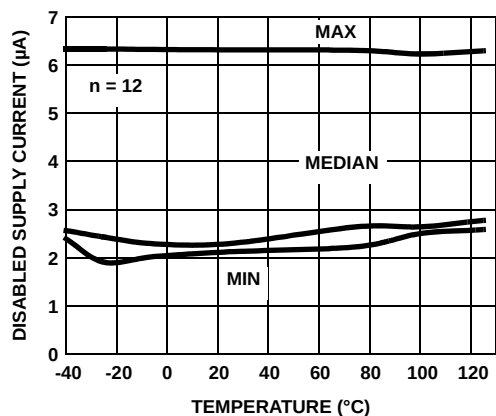
FIGURE 27. DISABLED SUPPLY CURRENT vs TEMPERATURE V_S = \pm 2.5V R_L = \text{INF}
