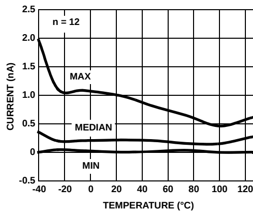
FIGURE 28. I_{\text{BIAS}} (+) vs TEMPERATURE V_S = \pm 2.5V
