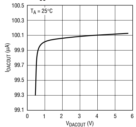
I_{DACOUT} FS vs V_{DACOUT} at V_{CC} = 5V
