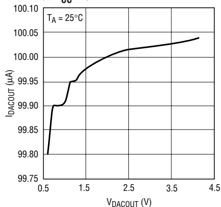
I_{DACOUT} FS vs V_{DACOUT} at V_{CC} = 3V
