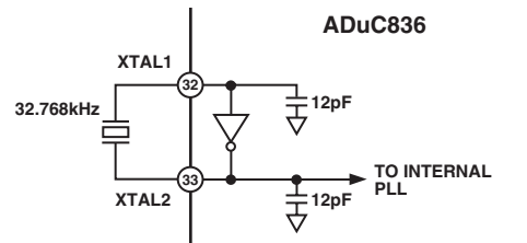
Figure 65. External Parallel Resonant Crystal Connections Other Hardware Considerations
