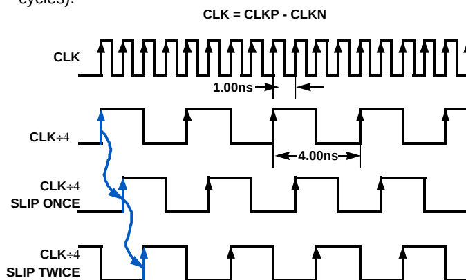
FIGURE 41. PHASE SLIP: CLK ÷ 4 MODE, f_{\text{CLOCK}} = 1000\text{MHz}
