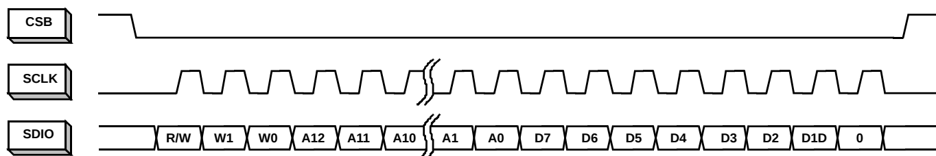
FIGURE 35. MSB-FIRST ADDRESSING
