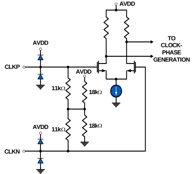
FIGURE 44. CLOCK INPUTS
