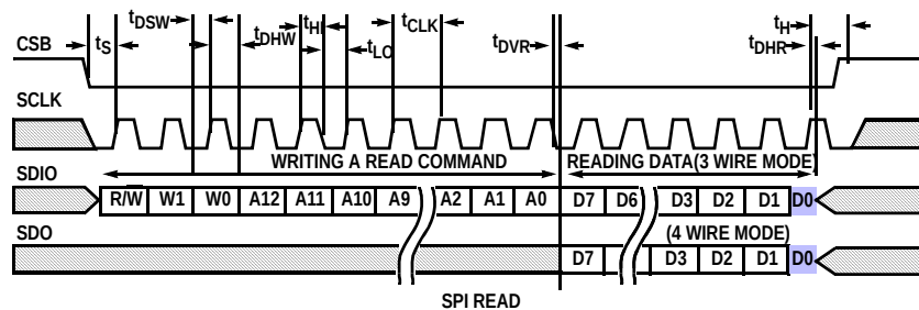
SPI READ FIGURE 38. READ TIMING
