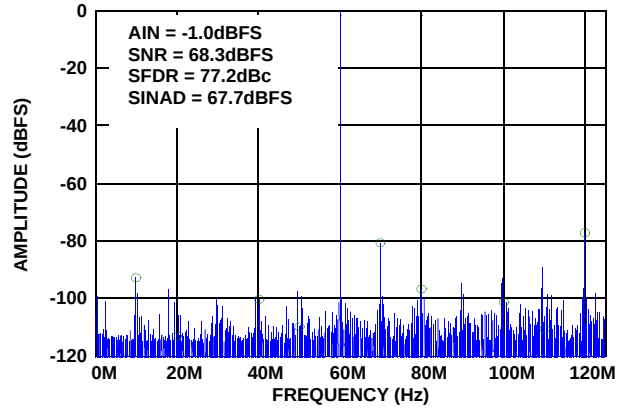
FIGURE 18. SINGLE-TONE SPECTRUM @ 190MHz
