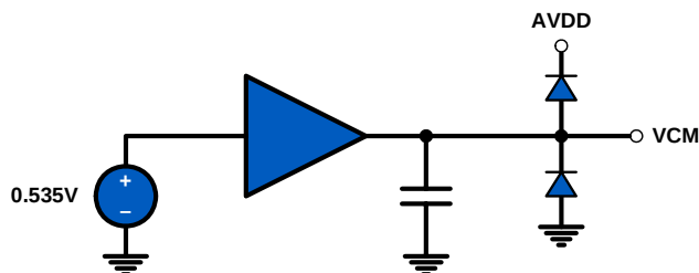
FIGURE 49. VCM_OUT OUTPUT
