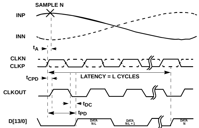
FIGURE 2B. SDR
