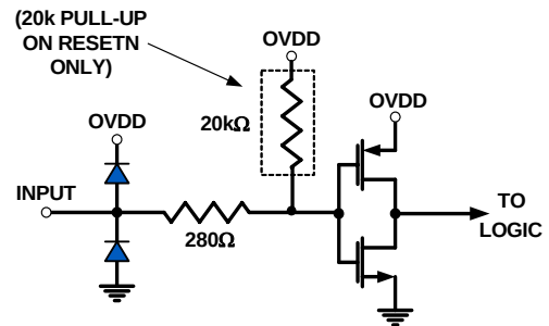
FIGURE 46. DIGITAL INPUTS
