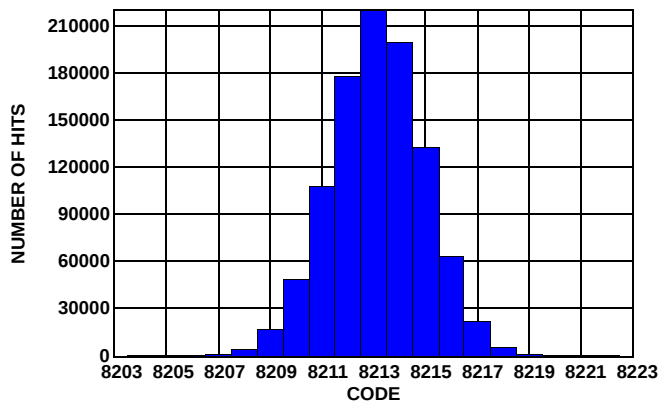
FIGURE 15. NOISE HISTOGRAM
