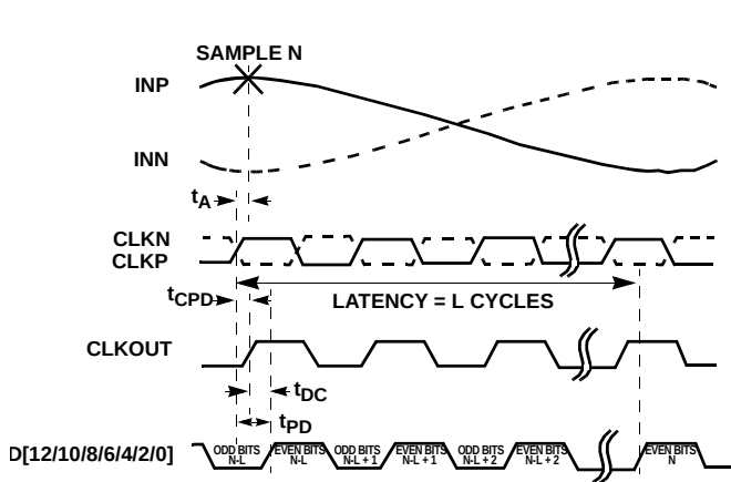
FIGURE 2A. DDR
