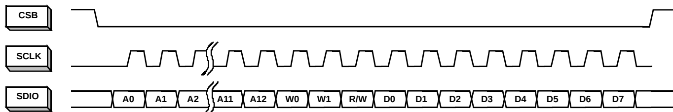
FIGURE 36. LSB-FIRST ADDRESSING
