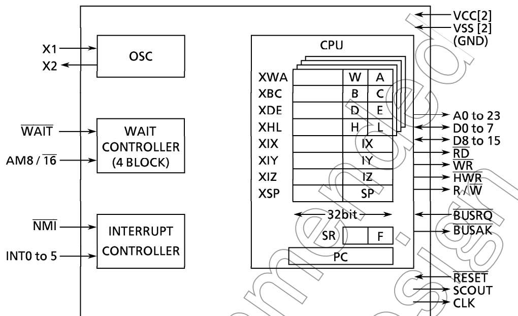
Figure 1 TMP95C001 Block Diagram
