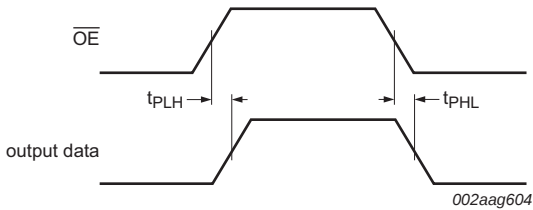
Fig 23. Output propagation delay
