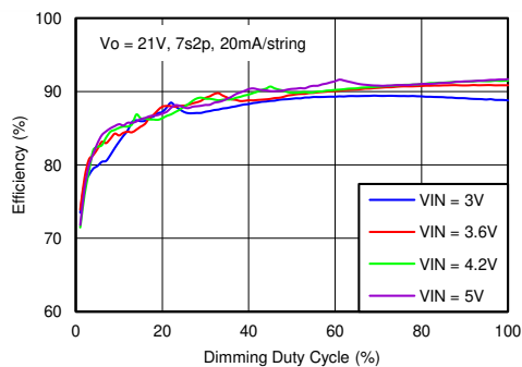
Figure 7-4. Dimming Efficiency
