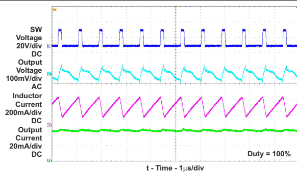
Figure 7-8. Switching Waveform
