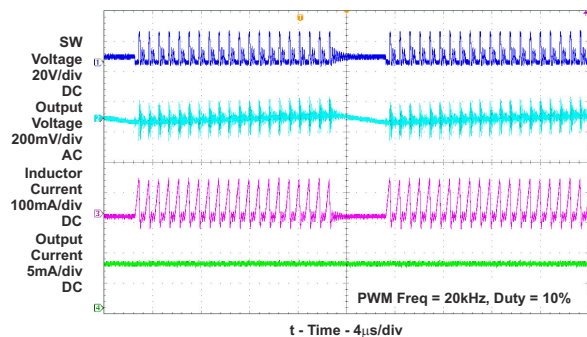
Figure 7-10. Switching Waveform
