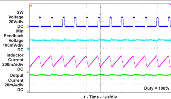
Figure 7-9. Switching Waveform
