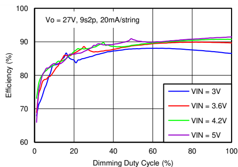
Figure 7-6. Dimming Efficiency
