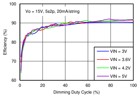
Figure 7-2. Dimming Efficiency
