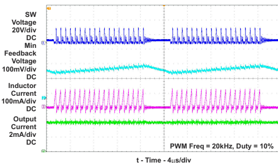
Figure 7-11. Switching Waveform
