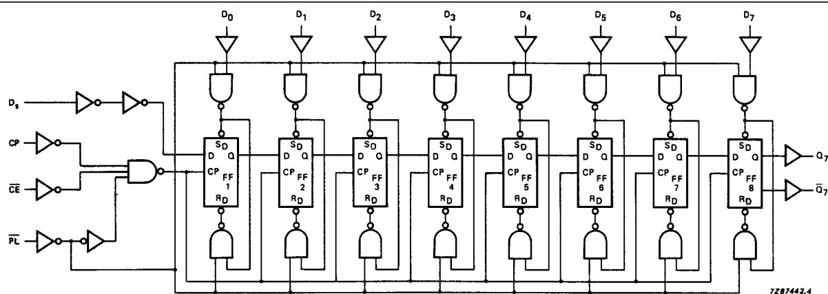
Fig.5 Logic diagram.
