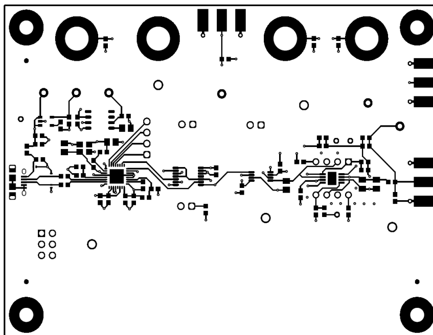
Figure 4-3. DAC8811EVM PCB Top Layer Layout
