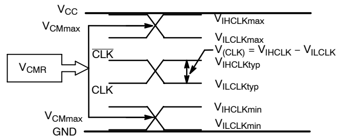
Figure 13. V_{CM} Diagram
