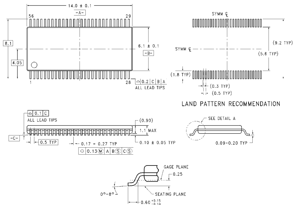
DETAIL A
