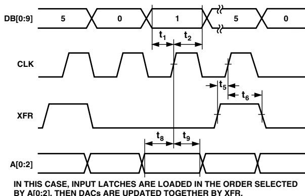
Figure 9. Addressed Channel Timing ( \overline{E/O} = HIGH, STSQ/CS = HIGH)
