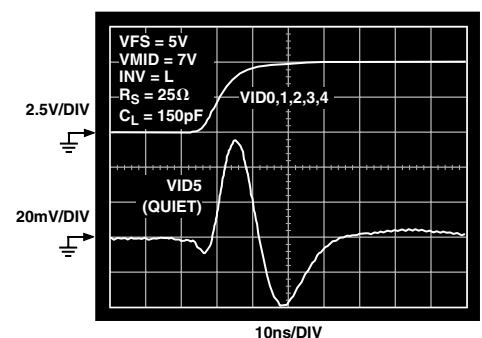
TPC 21. All-Hostile Crosstalk at C_L
