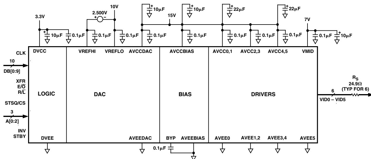
Figure 10. Interface Drawing
