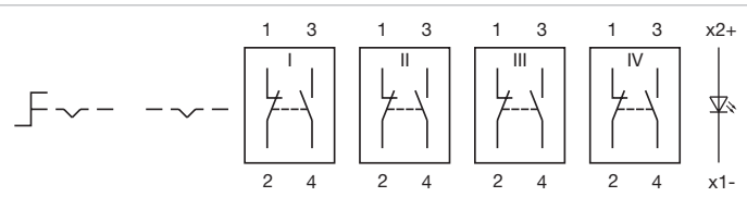
Wiring diagram 280
