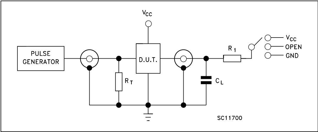
Figure 5. Test circuit 1
