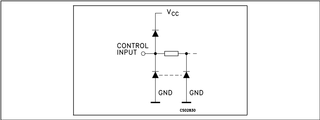
Figure 2. Control input equivalent circuit
