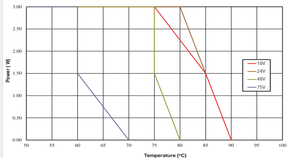
NCS3S4815SC
