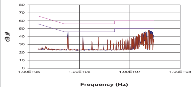
NCS3S1215SC
