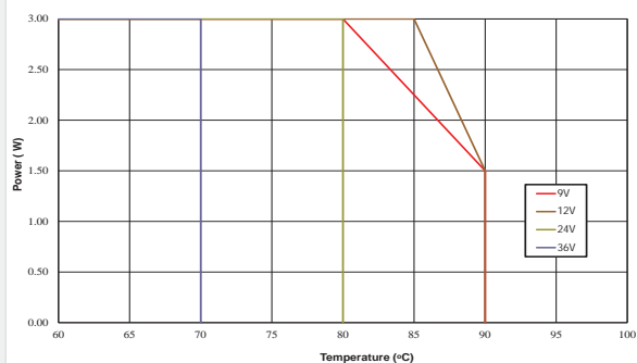
NCS3S4805SC
