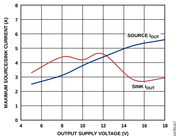
Figure 17. Maximum Source/Sink Current vs. Output Supply Voltage
