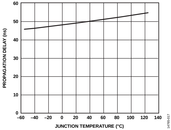
Figure 10. Propagation Delay vs. Junction Temperature
