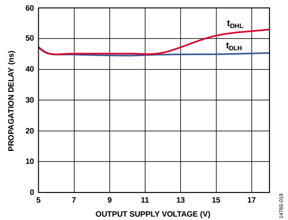
Figure 12. Propagation Delay vs. Output Supply Voltage, V_{DD1} = 5\text{ V}
