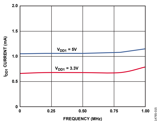
Figure 8. I_{DD1} Current vs. Frequency
