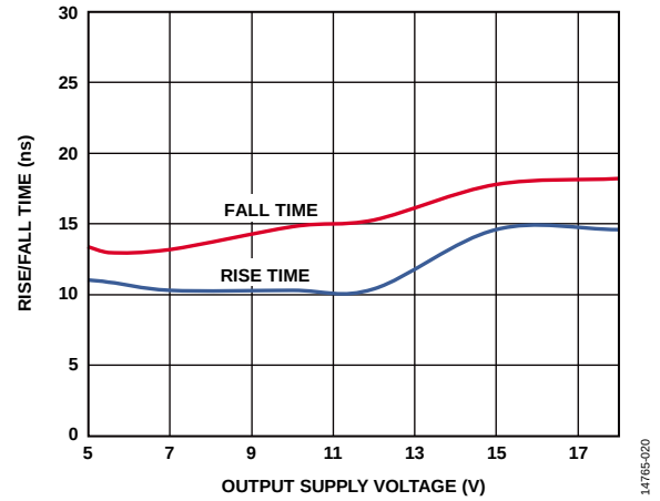
Figure 13. Rise/Fall Time vs. Output Supply Voltage
