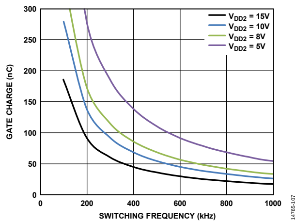
Figure 7. Maximum Load; Gate Charge vs. Switching Frequency ( R_{GATE} = 1 \Omega )
