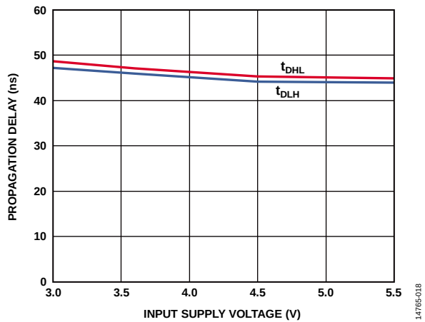
Figure 11. Propagation Delay vs. Input Supply Voltage, V_{DD2} = 10\text{ V}
