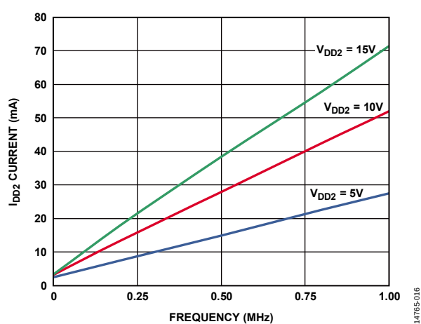
Figure 9. I_{DD2} Current vs. Frequency with 2 nF Load
