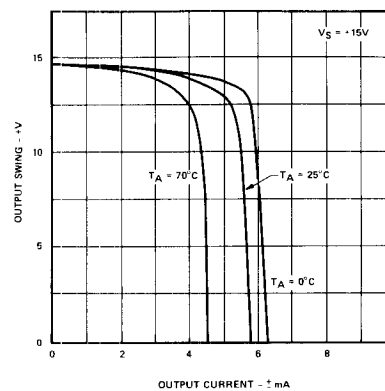
OUTPUT SWING
