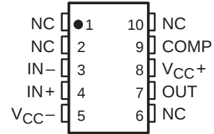
LM107 . . . U FLAT PACKAGE (TOP VIEW)
