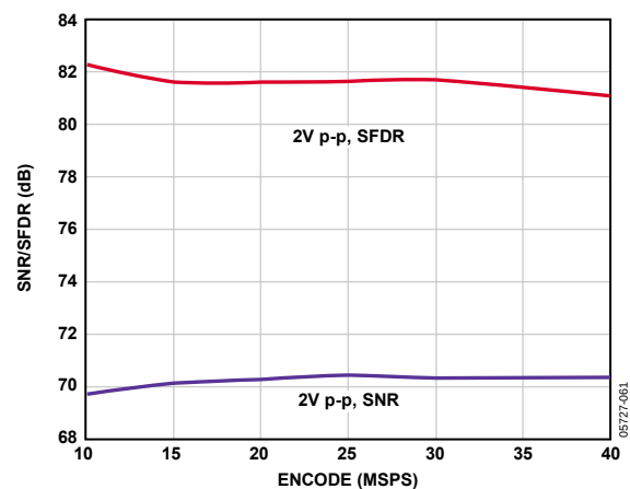
Figure 24. SNR/SFDR vs. f_{SAMPLE} , f_{IN} = 35 MHz, f_{SAMPLE} = 40 MSPS
