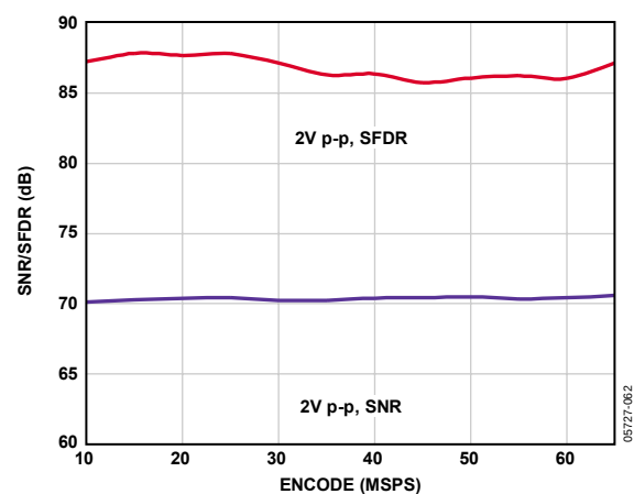
Figure 25. SNR/SFDR vs. f_{SAMPLE} , f_{IN} = 10.3 MHz, f_{SAMPLE} = 65 MSPS
