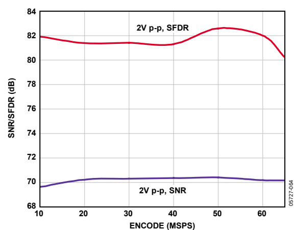
Figure 26. SNR/SFDR vs. f_{SAMPLE} , f_{IN} = 35 MHz, f_{SAMPLE} = 65 MSPS
