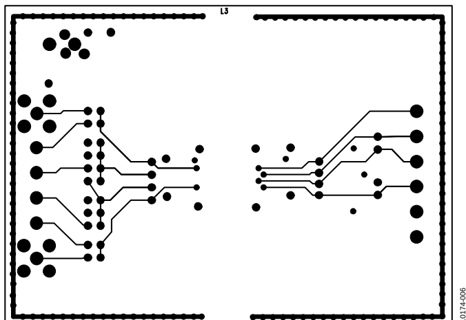
Figure 7. Internal Layer 3
