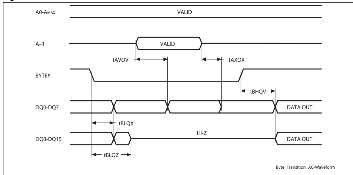
Figure 20. Page Read AC waveforms (16-bit mode)
