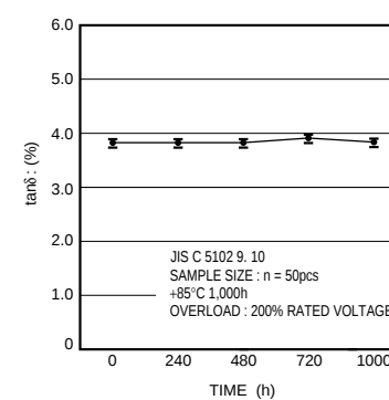
Fig.23 \tan\delta
