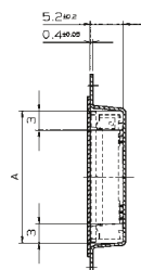
SECT. E-E
