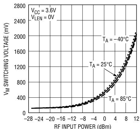
V_M Comparator Switching Voltage vs RF Input Power 5000MHz
