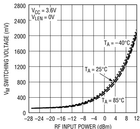
V_M Comparator Switching Voltage vs RF Input Power 4000MHz
