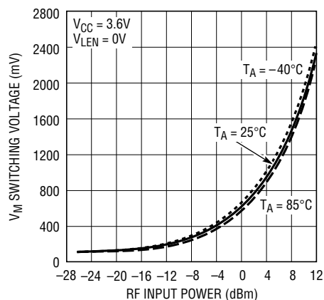
V_M Comparator Switching Voltage vs RF Input Power 1000MHz
