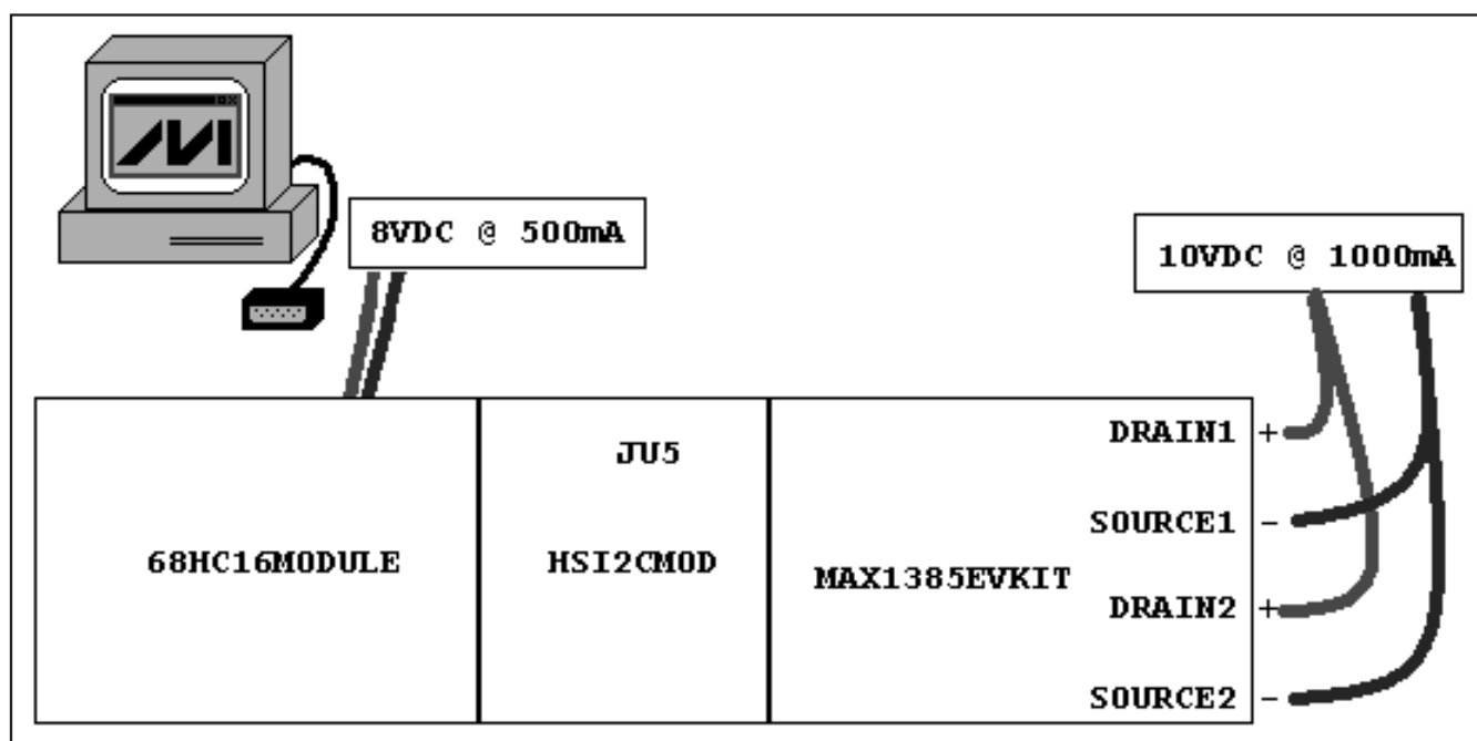
Figure 1. MAX1385 EV Kit System Connections
