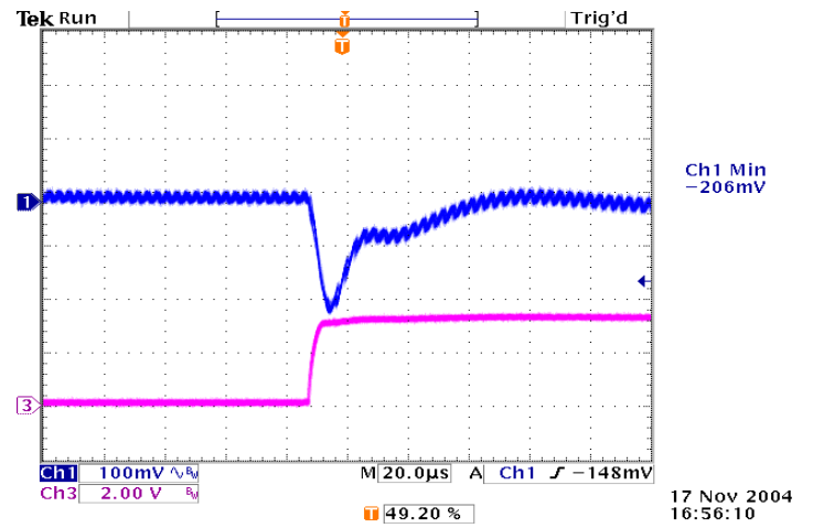
Figure 20: Typical transient response to step load change at 2.5A/\mu S from 50% to 100% of I_o , max at 5Vin, 3.3V out (Cout = ceramic, 10μF tantalum)
