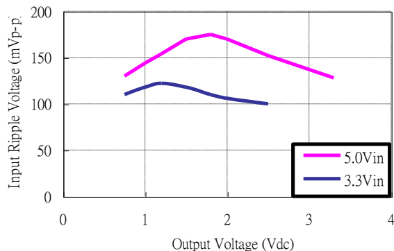
Figure 33: Input voltage ripple for various output models, IO = 16 A (CIN = 4x100 \mu F tantalum // 2x47 \mu F ceramic)
