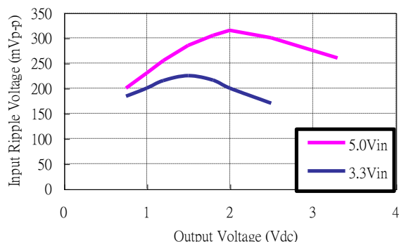
Figure 32: Input voltage ripple for various output models, IO = 16 A (CIN = 2x100 \mu F tantalum // 47 \mu F ceramic)
