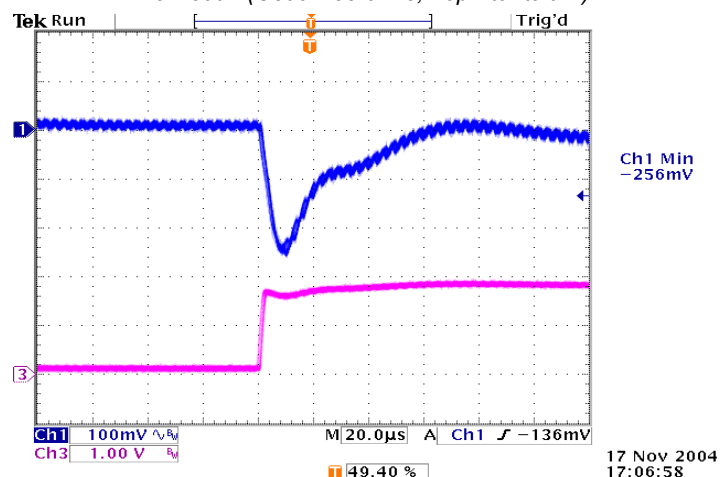
Figure 26: Typical transient response to step load change at 2.5A/ \mu s from 50% to 100% of I_o , max at 3.3Vin, 1.8V out ( C_{out} = ceramic, 10 \mu F tantalum)
