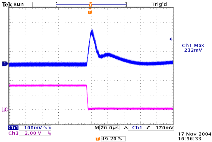
Figure 19: Typical transient response to step load change at 2.5A/\mu S from 100% to 50% of I_o , max at 5Vin, 3.3V out (Cout = ceramic, 10μF tantalum)
