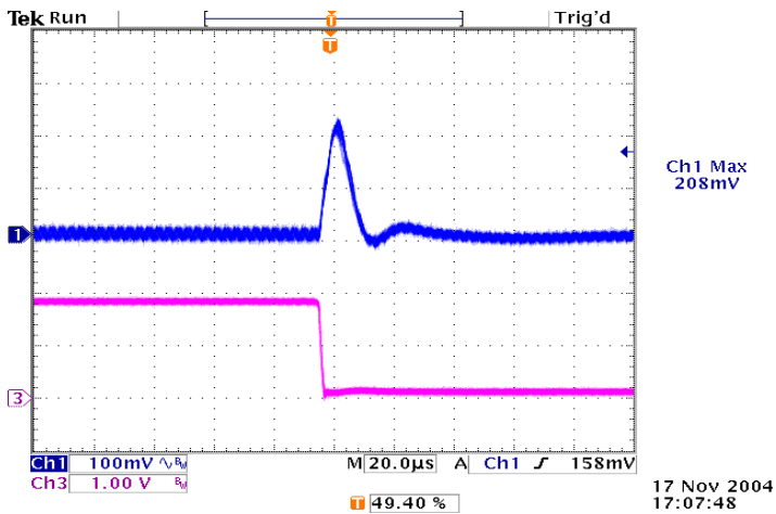
Figure 21: Typical transient response to step load change at 2.5A/\mu S from 100% to 50% of I_o , max at 5Vin, 1.8V out (Cout = ceramic, 10μF tantalum)
