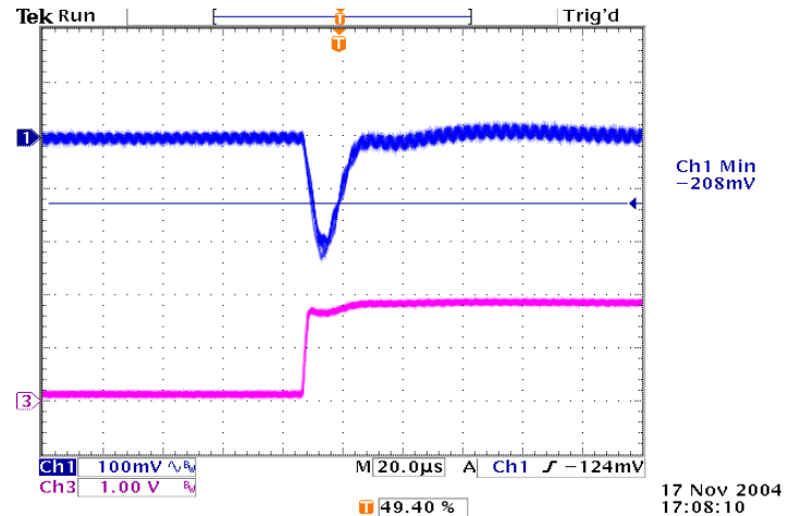
Figure 22: Typical transient response to step load change at 2.5A/\mu S from 50% to 100% of I_o , max at 5Vin, 1.8V out (Cout = ceramic, 10μF tantalum)
