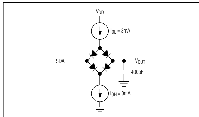
Figure 2. Load Circuit
