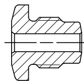
122835 DRIVING ANVIL -06
