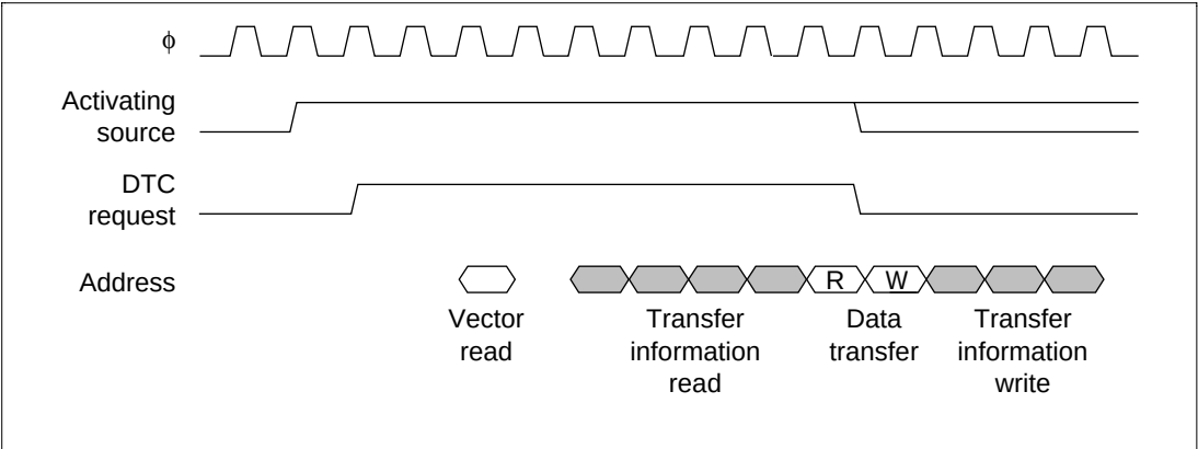
Figure 8.6 DTC Operation Timing Example (Normal Mode)
