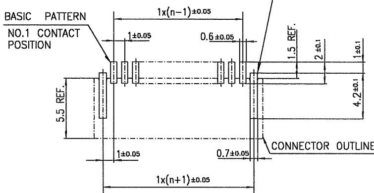
PATTERN FOR MOUNTING PLATE FIXING
