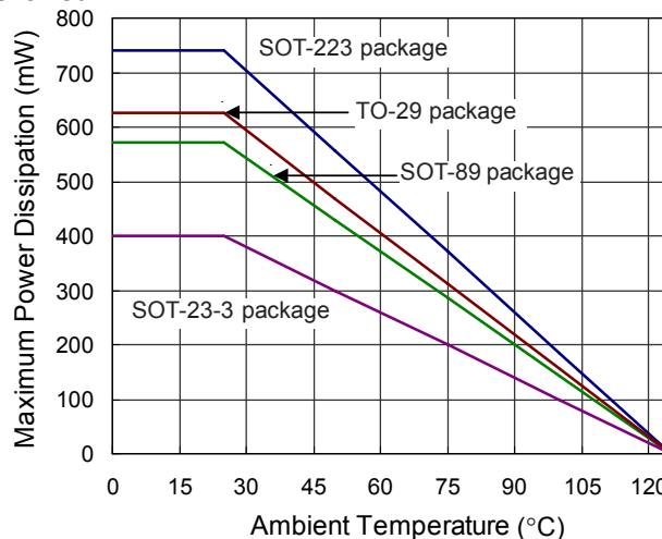
Figure 2. Derating Curves
