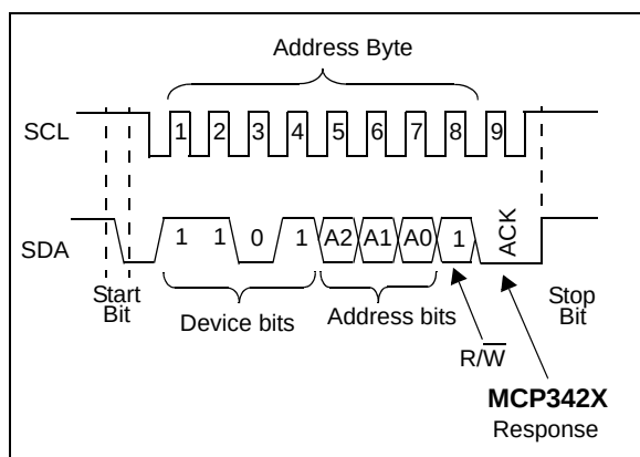
FIGURE 6-3: I 2 C Bus Connection Test.
