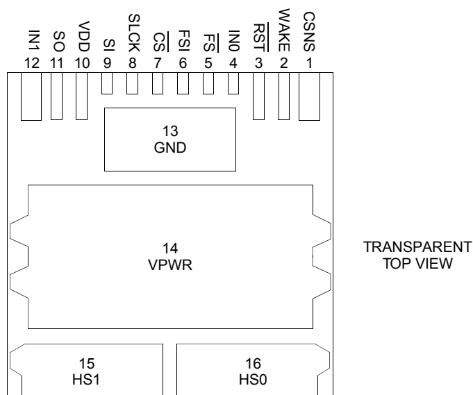
Figure 3. 33988 Pin Connections (Transparent Top View)
