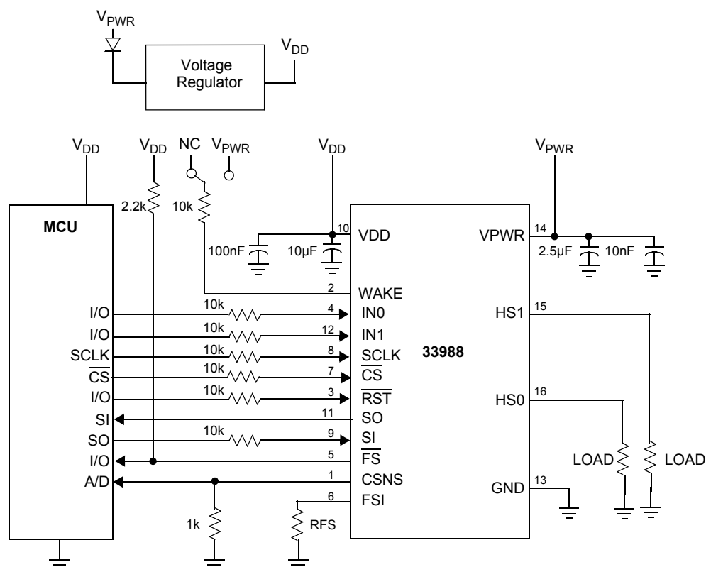
Figure 12. Typical Applications
