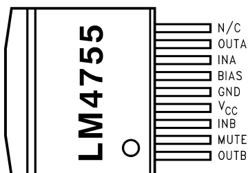
9 Pin DDPK Plastic Package (Top View) See Package Number KTW
