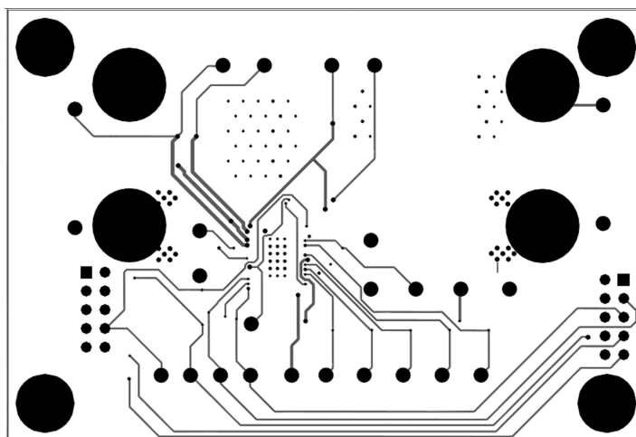
Figure 24. Board Mid Layer 2
