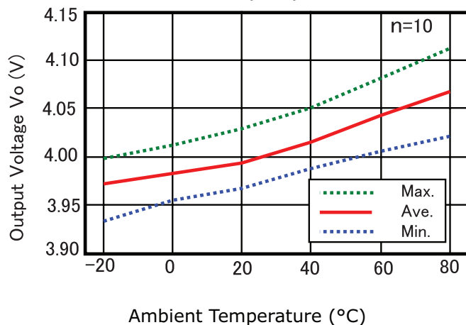
Output Voltage vs. Ambient Temperature [at +1f]
