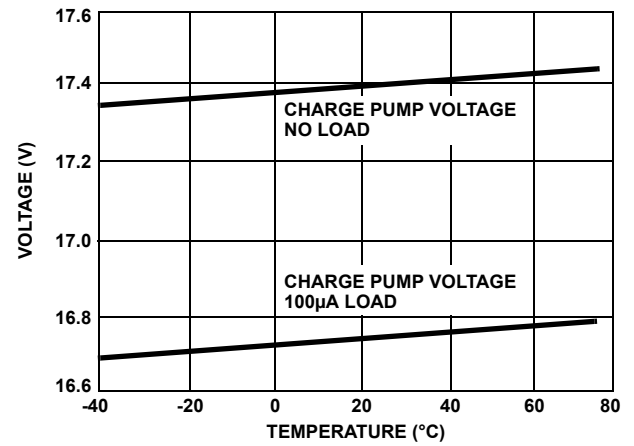
FIGURE 9. PUMP VOLTAGE
