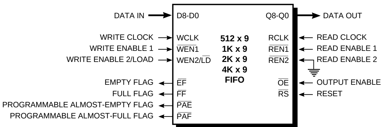
FIGURE 15. SINGLE-DEVICE MODE
