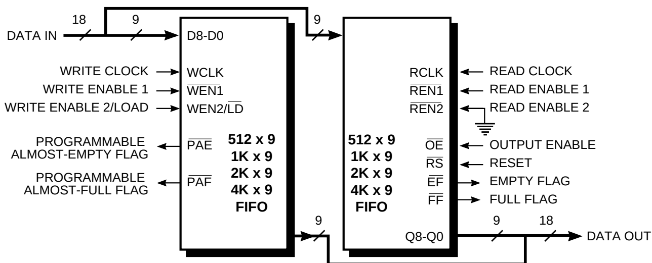
FIGURE 16. WIDTH-EXPANSION MODE
