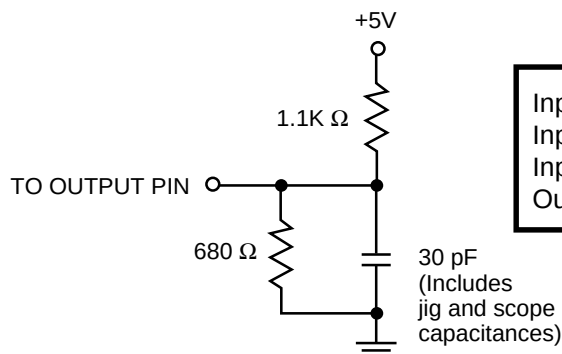
FIGURE 3. AC TEST CONDITIONS
