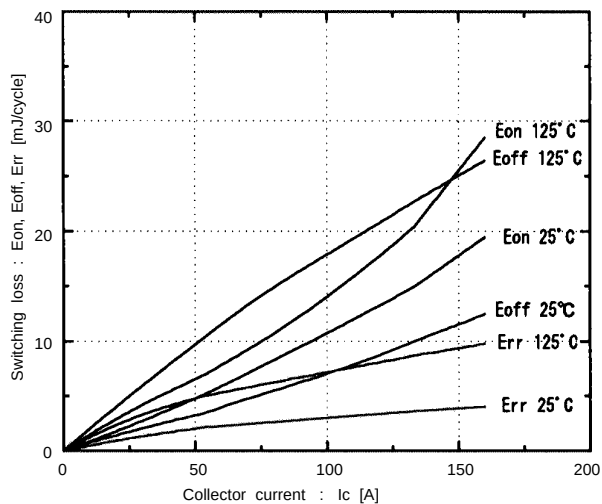
Switching loss vs. Collector current V_{CC}=600V , R_G=9.1\text{ ohm} , V_{GE}=\pm 15V
